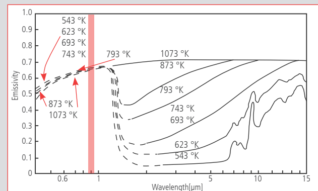
Emission of silicon as function of temperature and wavelength Quelle: Sato, T., Jap., Appl. Phys. 6, March, 1967, p. 339-347
